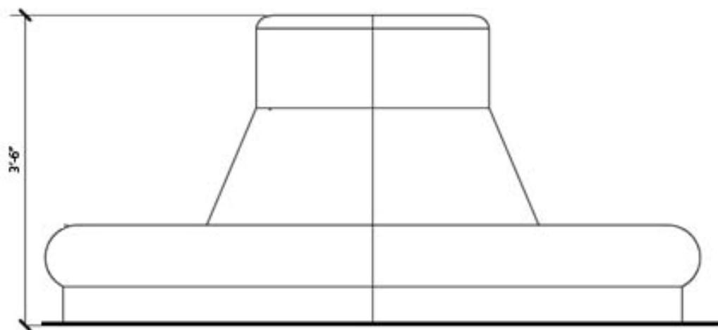
Elevation (NTS)
