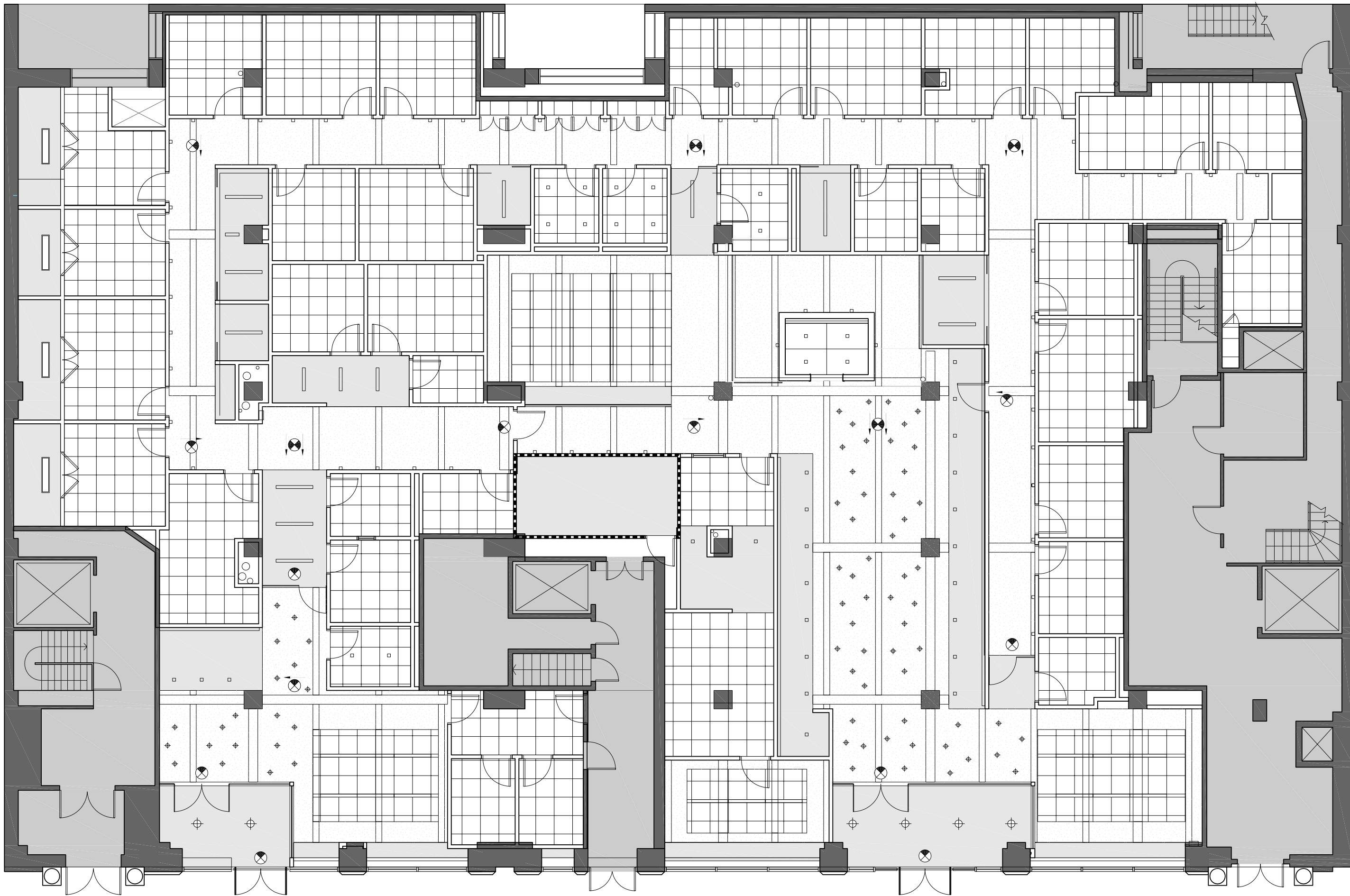
Ground Floor: Reflected Ceiling Plan
