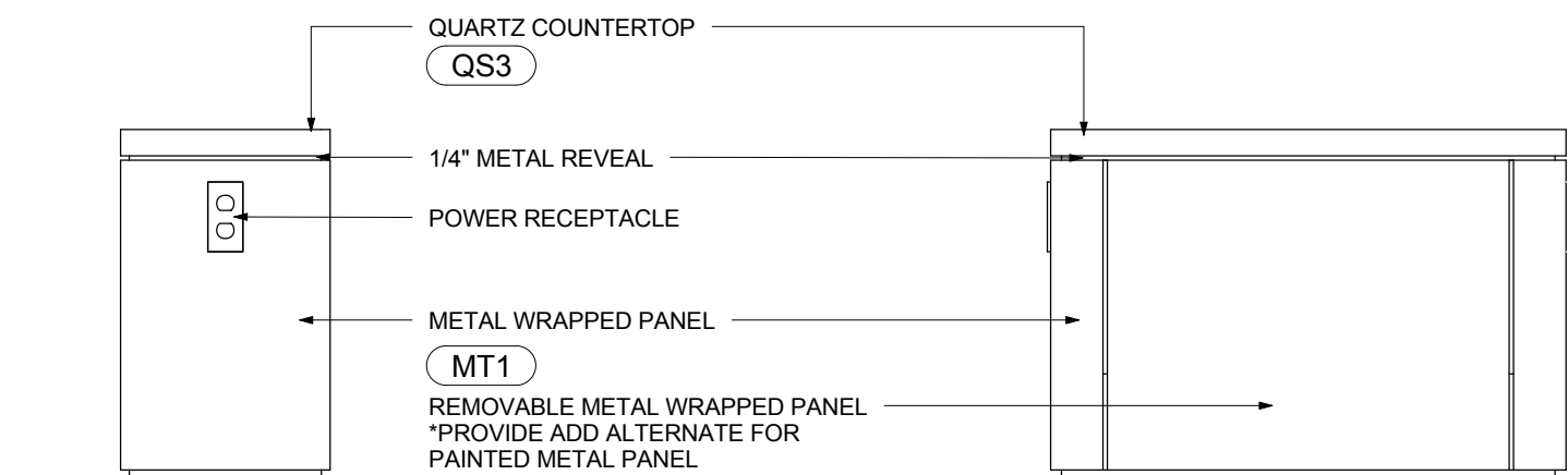
FRONT ELEVATION
